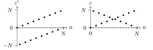
Figure 1. The dispersion relations (19) alternate between two linear branches, realising chiral and (up to a shift) ‘full’ massless relativistic dispersions on the lattice.
